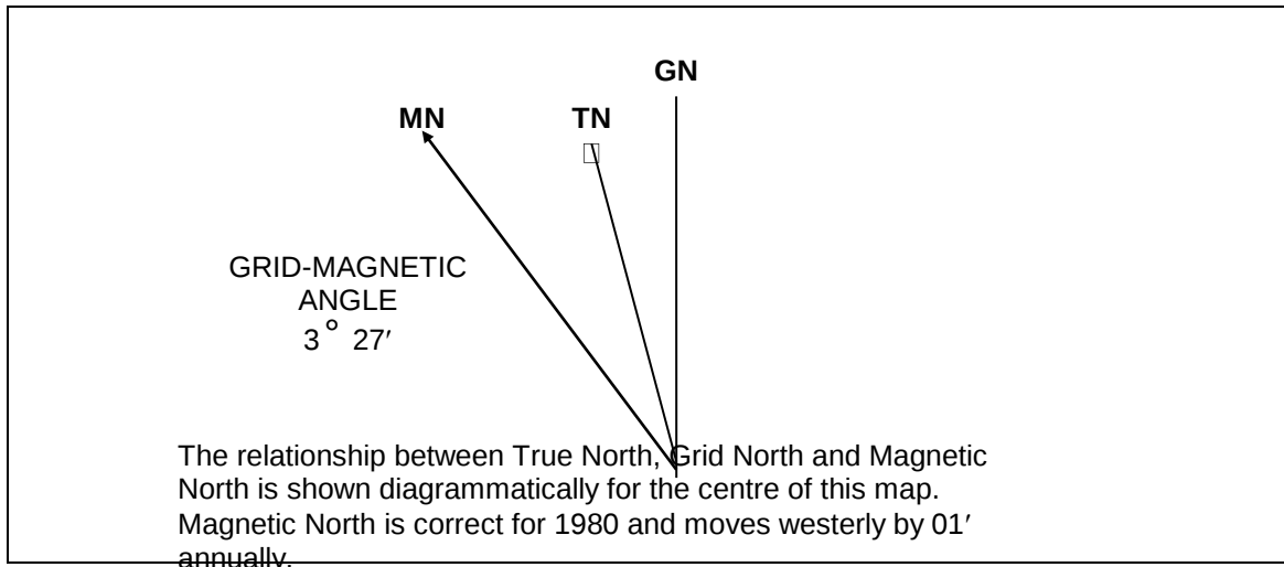
Figure 28 - Magnetic variation diagram
